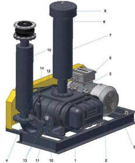
Type NVD-40 without outlet silencer
