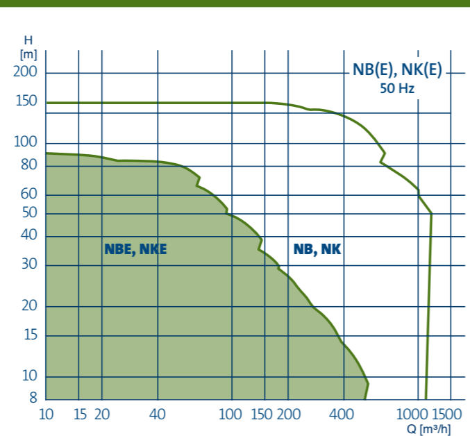
The curve shows the performance area of Grundfos end-suction pumps. The shaded area shows the performance area of pumps with integrated frequency converters (NBE/NKE pumps).
