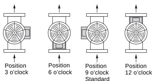
Fig. 28 Possible terminal box positions
