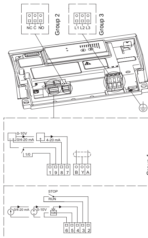
Fig. 33 Wiring diagram, three-phase TPE pumps
