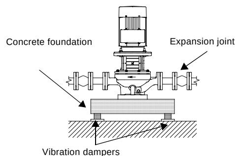
Fig. 24 Foundation of TP pump
