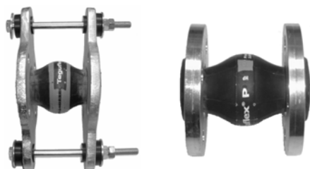
Fig. 26 Examples of rubber bellows expansion joints
