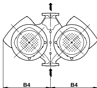
Fig. 29 Terminal box positions of TPED pumps
