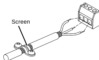
Fig. 30 External start/stop cable connection of TPE, TPED
