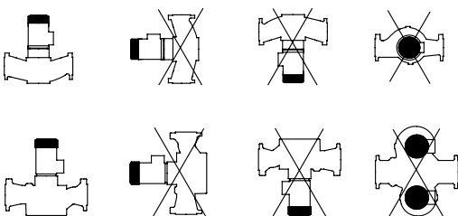
Fig. 19 Installation of motor sizes of 11 kW and up
