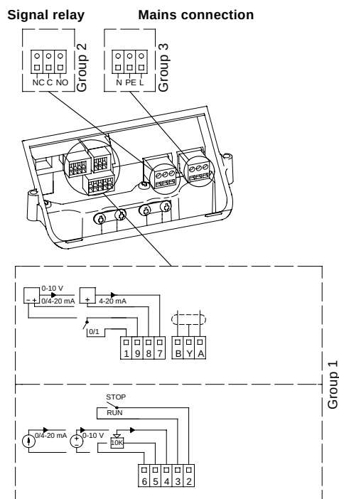
Fig. 32 Wiring diagram, single-phase TPE pumps
