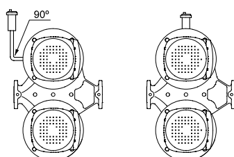
Fig. 20 Twin-head pumps with automatic air vent
