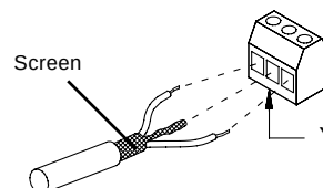
Fig. 31 Bus connection of TPE, TPED
