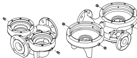
Fig. 21 Tappings for mounting of automatic air vents in TP Series 200 and TP Series 300
