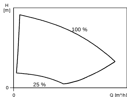
Fig. 12 Duty range of TPE Series 2000 pumps
