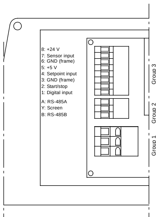
Fig. 34 Wiring diagram, three-phase TPE pumps
